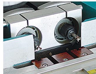
Router units with spindle spacing 65 mm
